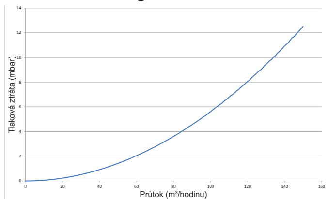
MagnaClean 8"
